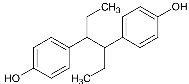
diethylstilbestrol (trans!)
