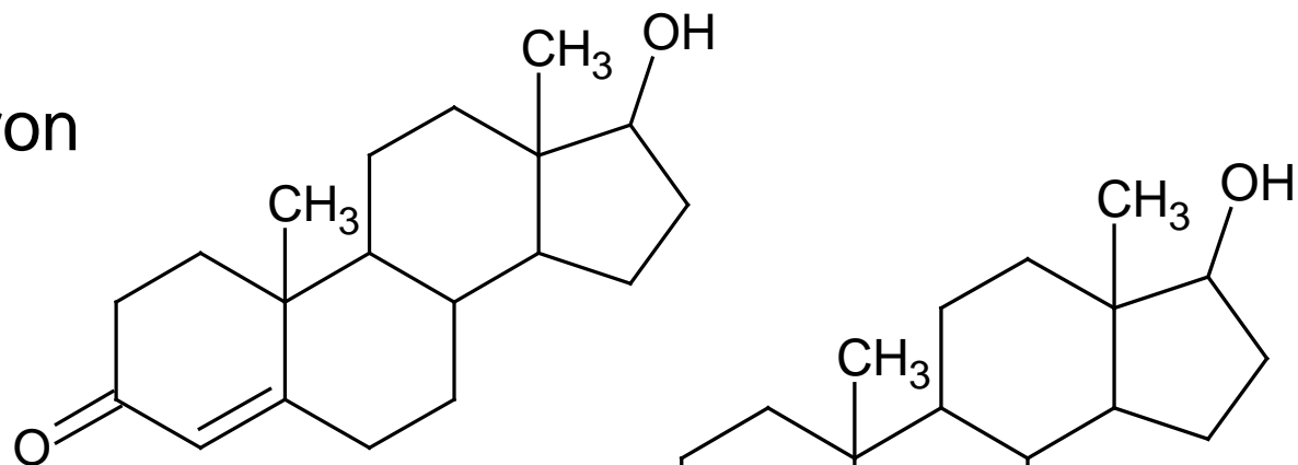
Dihydrotestosteron
