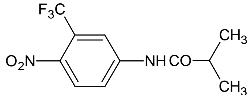
flutamid
